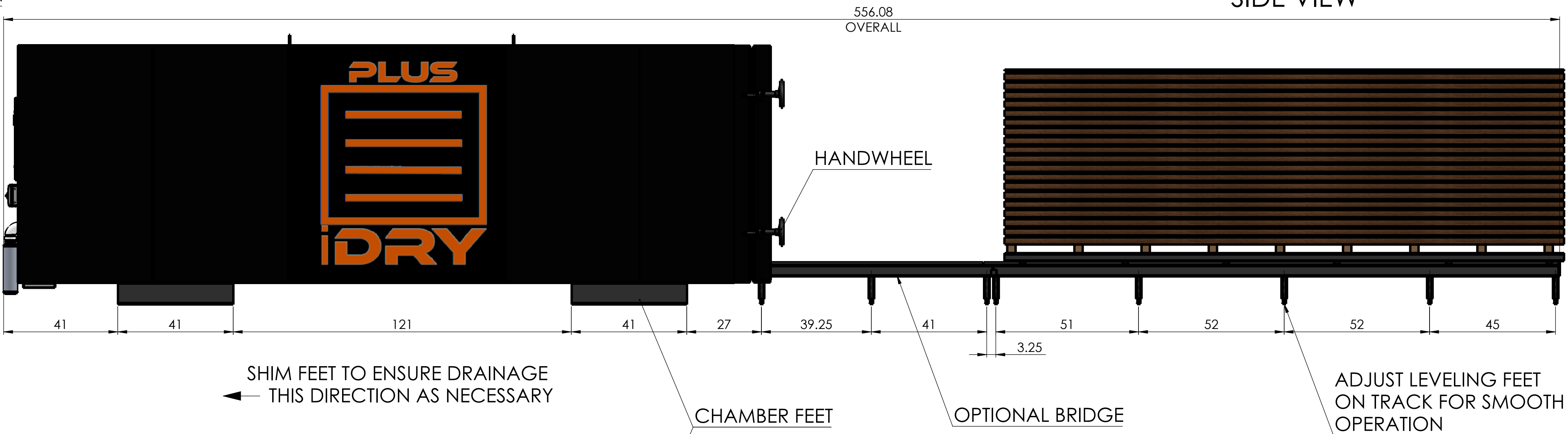
SIDE VIEW
